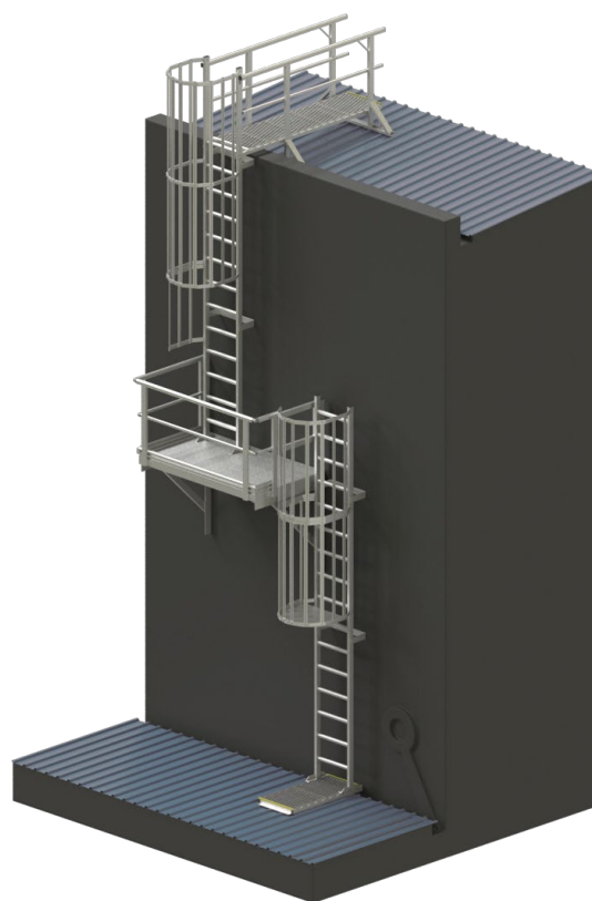
ROOF SHEETING TO ROOF SHEETING Below Drawing: LADERK002.171+FOOTING
