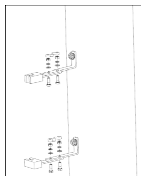
Installed with Cable Guide Pole Support Bracket Extended 100mm PC:VLINE.PLT.CG.EXT
