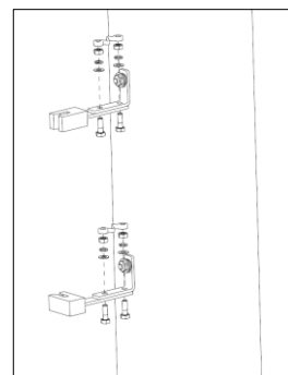
Installed with Cable Guide Pole Support Bracket PC:VLINE.PLT.CG
