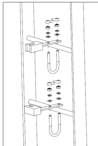
Installed to Ladder Rungs Top Pic: Straight Cable Guide Bottom Pic: 90 Degree Cable Guide
