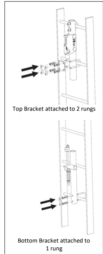
Bottom Bracket
