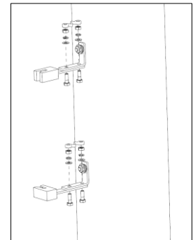
Installed with Cable Guide Pole Support Bracket PC:VLINE.PLT.CG
