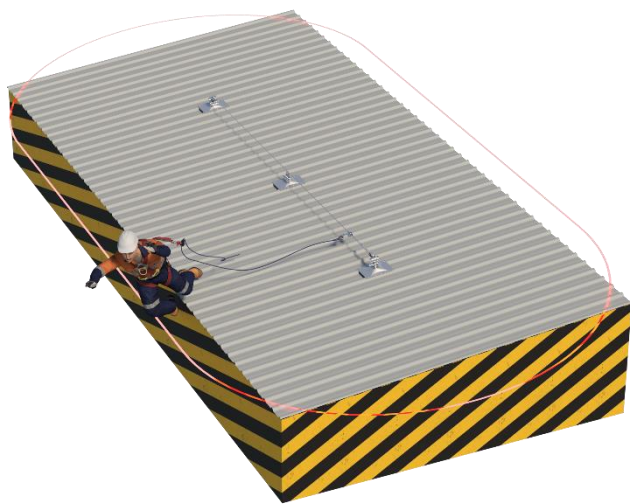
Free fall: Freefall distance greater than 600 mm.
