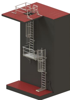
Kit: LADERK002.164+FOOTING PLATFORM
