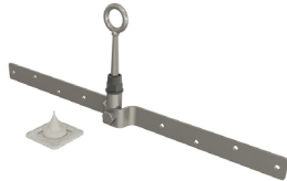
SafetyLink Side Mounted RafterLink
